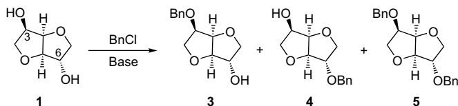
Scheme 1. Benzylation of isosorbide.
