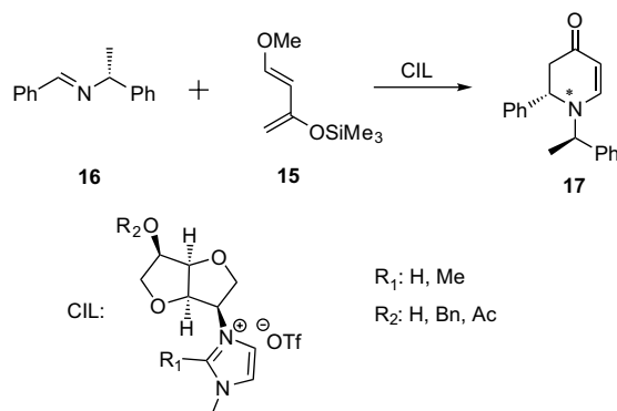
Scheme 5. Asymmetric aza Diels–Alder reaction of Danishefsky's diene 15 with imine 16 .
