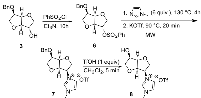
Scheme 2. Synthesis of imidazolium salts 7 and 8 .
