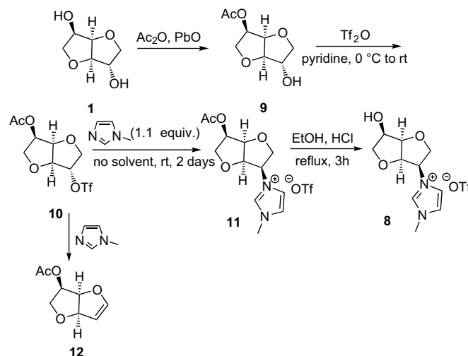
Scheme 3. Synthesis of imidazolium salt 8 .
