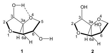
Figure 1. Structure of isosorbide 1 and isomannide 2 .
