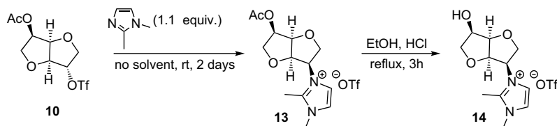
Scheme 4. Synthesis of CIL 14 .
