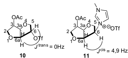
Figure 2. Inversion of configuration confirmed by ^1\text{H} NMR.
